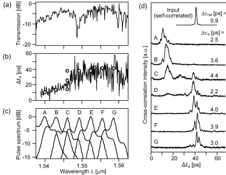
Fig. 5. Transmission characteristics of PCCW. (a) Transmission spectrum. (b) Group delay characteristics measured by using modulation phase shift method. Circular plots show the delay obtained from those of optical pulse in (d). (c) Input pulse spectra. (d) Cross-correlation traces of output pulse and reference pulse. The top shows the auto-correlation trace of input and reference pulses. Pulse width \Delta\tau_o was estimated by deconvoluting the cross-correlation trace of the output pulse from the reference pulse. In (b)–(d), A–G denote the same pulse spectra.
