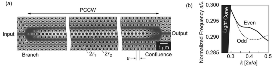
Fig. 3. PCCW integrated with input/output PCW. (a) Top view of fabricated device on SOI substrate. 2r_1 is chirped from 0.25 \mu\text{m} to 0.27 \mu\text{m} . 2r_2 is fixed at 0.36 \mu\text{m} . (b) Photonic band diagram of PCCW.
