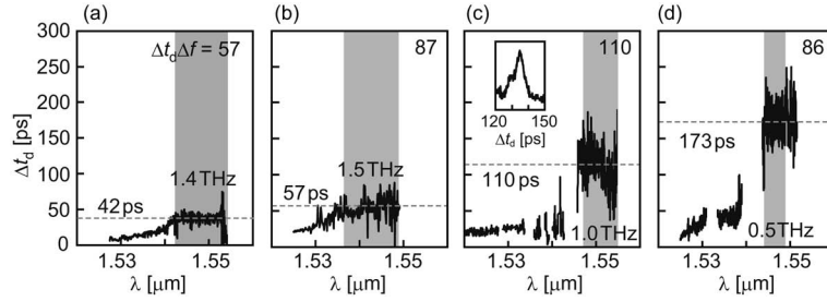
Fig. 6. Delay spectra observed for L = (a) 250 \mu\text{m} , (b) 400 \mu\text{m} , (c) 800 \mu\text{m} , and (d) 1 mm. Discontinuity of spectra in (c) and (d) is due to low output power that disturbed the acquisition of reliable data. Gray bands denote the effective slow light band, in which moving average of data points is lying inside \pm 10\% of the total average value. Gray dashed lines denote average delay in the effective band. The inset in (c) shows the cross-correlation trace of optical pulse with \Delta\tau_{\text{ref}} = 0.9 ps and \Delta\tau_o = 5.5 ps. As the center wavelength of the pulse was set at 1.549 \mu\text{m} , \Delta t_d increases from the average value indicated by the gray dashed line to 130 ps.
