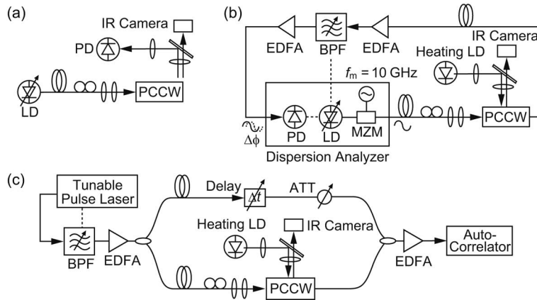
Fig. 4. Measurement setups for (a) transmission spectrum, (b) group delay spectrum using modulation phase shift method, and (c) pulse transmission.
