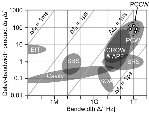
Fig. 1. Relation of delay-bandwidth product and bandwidth of slow light from various sources. Circular plots of PCCW correspond to experimental results in Fig. 6.
