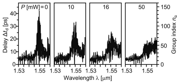
Fig. 7. Change of the delay and group index spectra against local heating at the branch of unchirped PCCW ( 2r_1 = 0.25 \mu\text{m} ), which was observed in modulation phase shift measurement.
