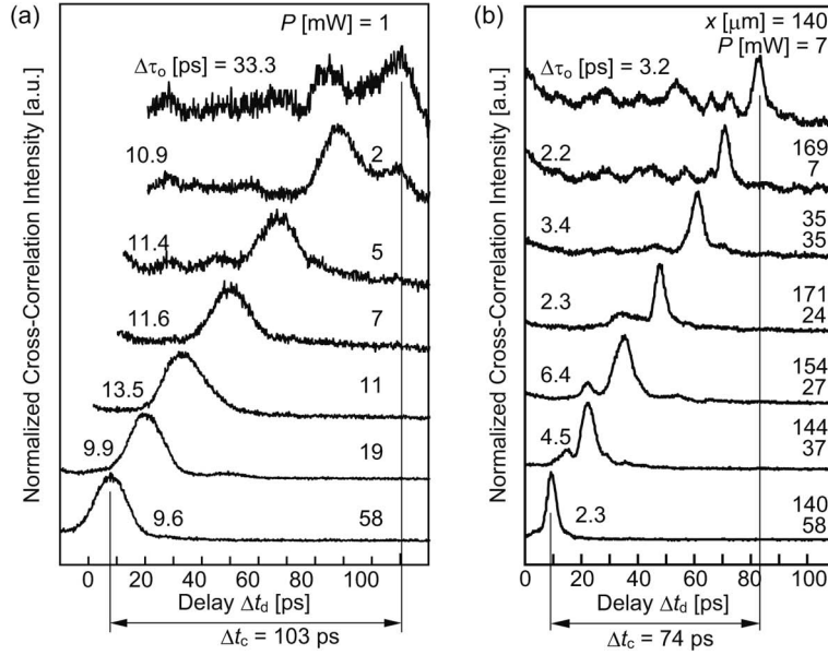
Fig. 10. Delay tuning of different width slow light pulse. For (a), the center position of the heating, x , is fixed at the center of PCCW, i.e. 140 \mu\text{m} .
