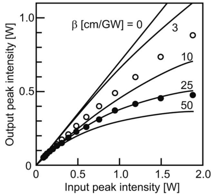
Fig. 12. Intensity response of zero-dispersion PCW. Solid lines are the calculation results for different effective TPA coefficients \beta . The open and closed circles denote the experimental results for two PCWs exhibiting n_g \sim 8 and 30, respectively.
