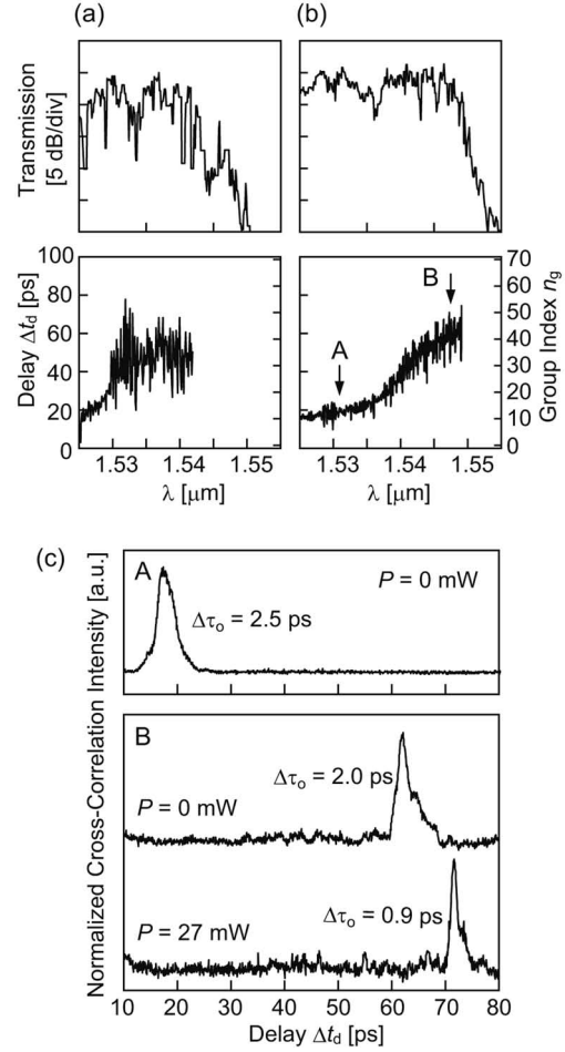
Fig. 9. Slow light characteristics of 400- \mu\text{m} -long chirped PCCW. (a) Transmission and delay spectra of monotonous-chirped device, and (b) those of folded-chirped device. (c) Normalized cross-correlation trace of output pulse, where A and B correspond to those in (b).
