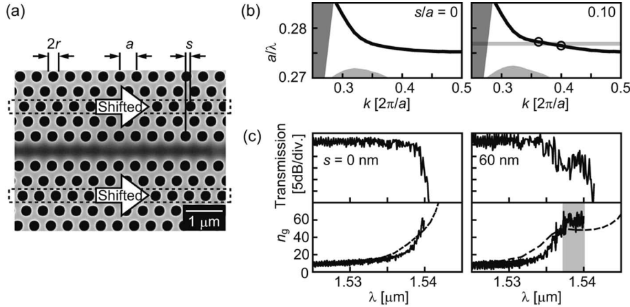
Fig. 11. Low-dispersion slow light. (a) Top view of fabricated lattice-shifted PCW showing zero-dispersion slow light. (b) Calculated two-dimensional band of the guided mode for two s/a with an equivalent index of 2.9 and the transverse-electric polarization. The gray line and circles denote zero-dispersion slow light. (c) Measured transmission characteristics for two s . The gray region and dashed line denote zero-dispersion slow light and the calculated group index, respectively.
