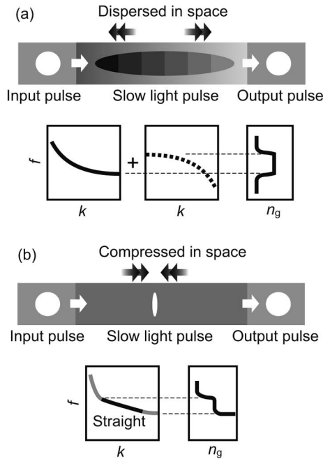
Fig. 2. Schematics of two types of wideband dispersion-free slow light. (a) Dispersion-compensated slow light. (b) Low-dispersion slow light.
