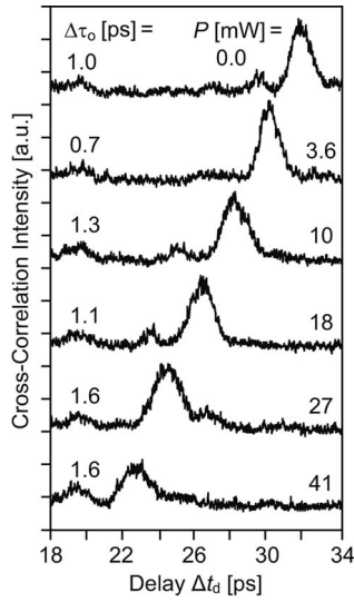
Fig. 8. Cross-correlation trace of output optical pulse from the chirped PCCW against local heating.
